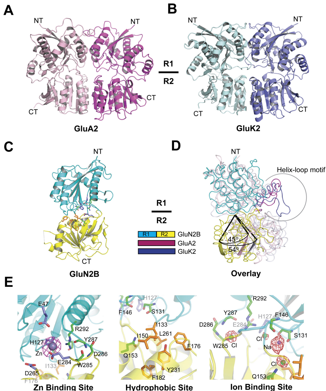
Fig. 2. Structures of ionotropic glutamate receptor ATDs. A , structure of the AMPA receptor GluA2 ATD dimer (PDB code 3H5V). The ATD structure adopts a bilobed structure composed of two halves, referred to as R1 (distal to the membrane) and R2 (proximal to the membrane), with extensive intersubunit R1-R1 and R2-R2 contacts. The N terminus is located at the top of the R1 lobe, whereas the bottom of the R2 lobe connects to the ligand binding domain through the ATD-S1 linker. B , the structure of the kainate receptor GluK2 ATD (PDB code 3H6G) is similar to that of the GluA2 ATD. C , the GluN2B ATD is also a clamshell-like bilobed structure composed of two halves (R1 in blue and R2 in yellow) (PDB code 3JPY). D , structural alignment of the ATD structures from GluN2B and non-NMDA receptors (GluA2/GluK2). The GluN2B ATD has a structural fold similar to that of non-NMDA receptor ATDs but with a strikingly different conformation. The position of the R1 lobe in the GluN2B ATD is rotated \sim 50^\circ relative to the R2 lobe compared with the ATDs from AMPA and kainate receptors. This “twisted” R1-R2 orientation of GluN2B ATD results from the lack of a helix-loop motif present in both AMPA and kainate receptors, which hold R1 and R2 lobes together in a “nontwisted” configuration. E , evaluation of the GluN2B ATD structure reveals possible modulatory binding sites. The cleft between the R1 and R2 lobes contains a hydrophilic pocket with polar residues that participate in \text{Zn}^{2+} coordination, a hydrophobic pocket that resides deeper in the cleft containing some (but not all) residues critical for activity of the GluN2B-selective antagonist ifenprodil, and an ion binding site that accommodates one \text{Na}^+ and three \text{Cl}^- ions. Density for \text{Zn}^{2+} is represented by anomalous difference Fourier map at 6\sigma whereas that for \text{Na}^+ and \text{Cl}^- is represented by F_o - F_c omit map at 5.5\sigma .
