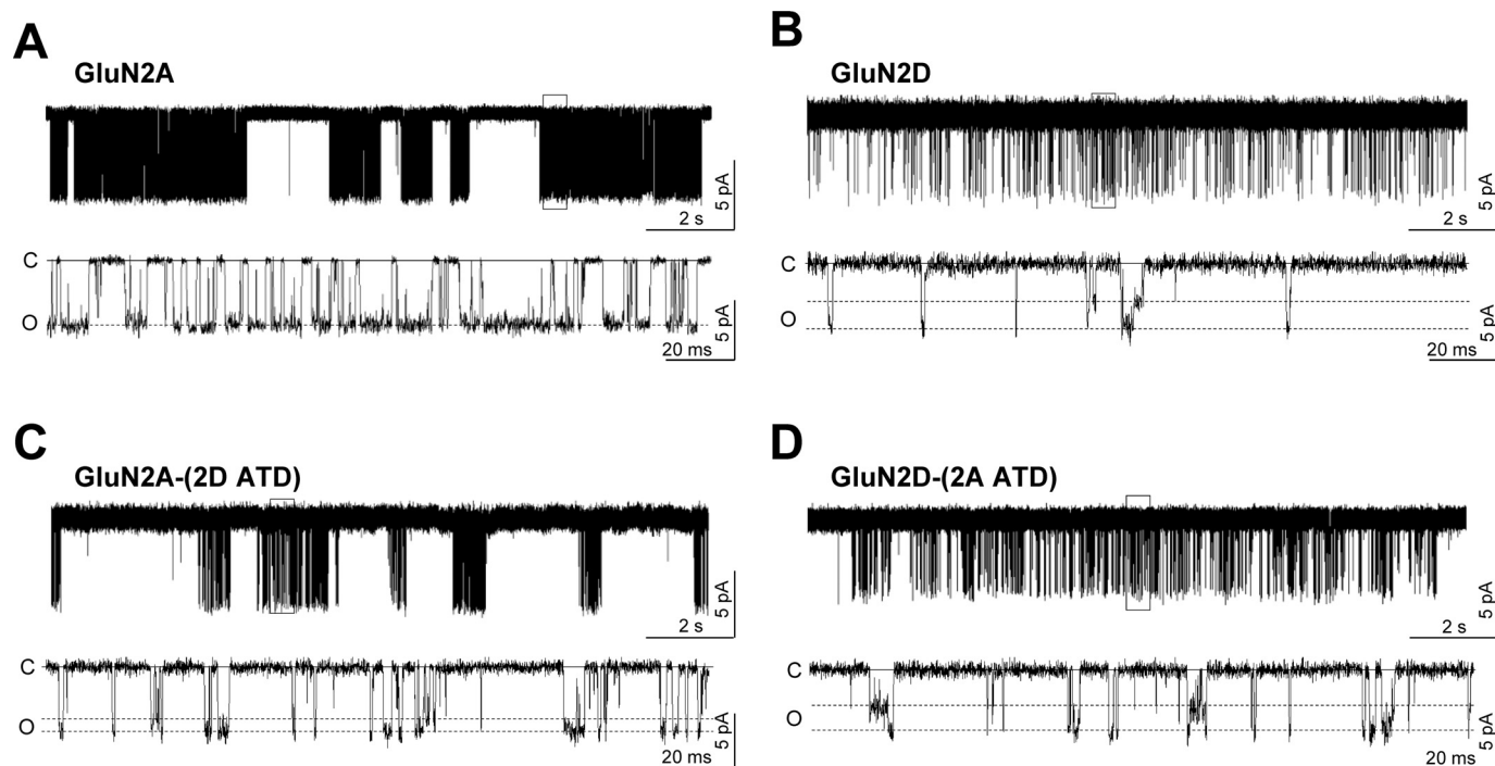
Fig. 4. The NMDA receptor subunit GluN2 ATD influences open probability. Exchange of the ATD between GluN2A and GluN2D shifts the open probability in the direction of the subunit contributing the ATD without changing the channel conductance. Replacement of the GluN2A ATD with that of GluN2D decreases open probability and mean open duration. By contrast, replacement of the GluN2D ATD with that of GluN2A increases open probability and mean open duration. Wild-type and chimeric GluN2 subunits were coexpressed with GluN1 in human embryonic kidney cells and characterized by recordings from single channels in outside-out patches in the presence of saturating glutamate and glycine. See also Fig. 3. [Reproduced from Yuan H, Hansen KB, Vance KM, Ogden KK, and Traynelis SF (2009) Control of NMDA receptor function by the NR2 subunit amino-terminal domain. J Neurosci 29:12045–12058. Copyright © 2009 The Society for Neuroscience. Used with permission.]
